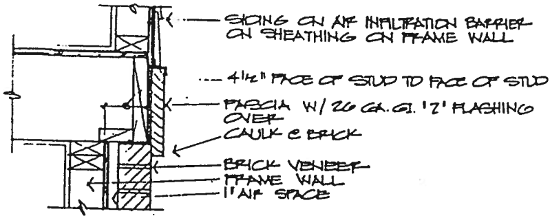
BRICK VENEER DETAIL 0 3' 0" 12'
