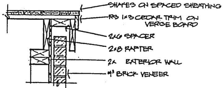
VERGE & BRICK VENEER
