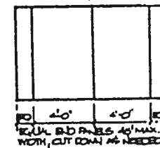
CONCEPTUAL SCREEN PATTERNS 1/2"=1'-0" OPTIONAL 4x8 PANEL CONFIGURATIONS
