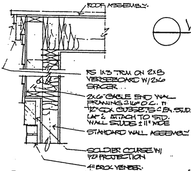
GABLE END
