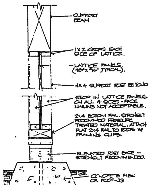
TYPICAL DECK DETAIL 3/4"=1'-0"
